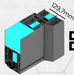
Deluxe Curved Door Systems
